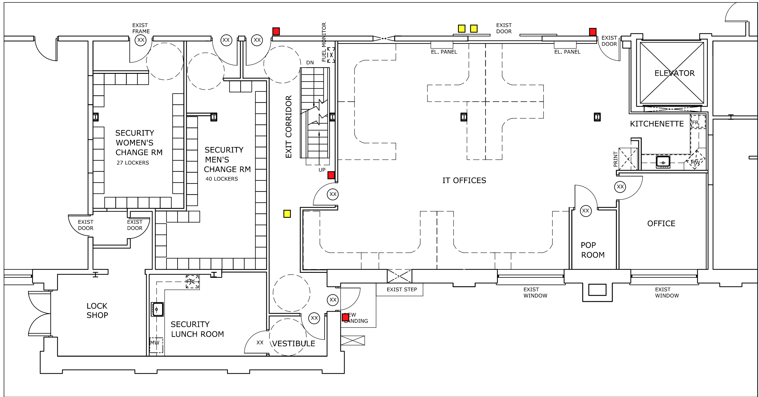
2 PARTIAL MAIN FLOOR PLAN — PROPOSED PLAN A1 SCALE: 1/8"=1'-0"
